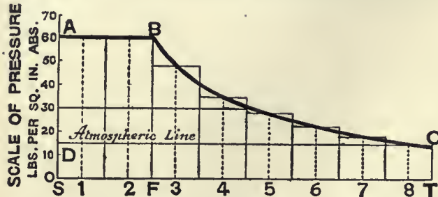
FIG. 3.—Watt's Indicator Diagram. Patent of 1782.
